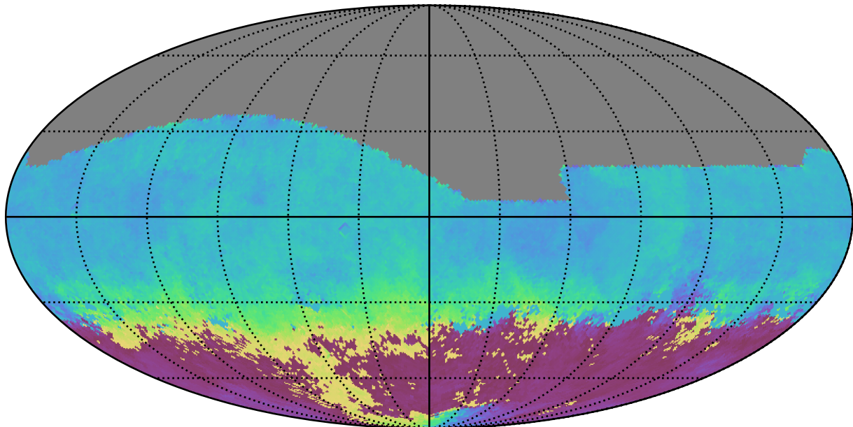
scp_reweight_v3.3_10yrs All sky g band: AngleMean rotSkyPos
