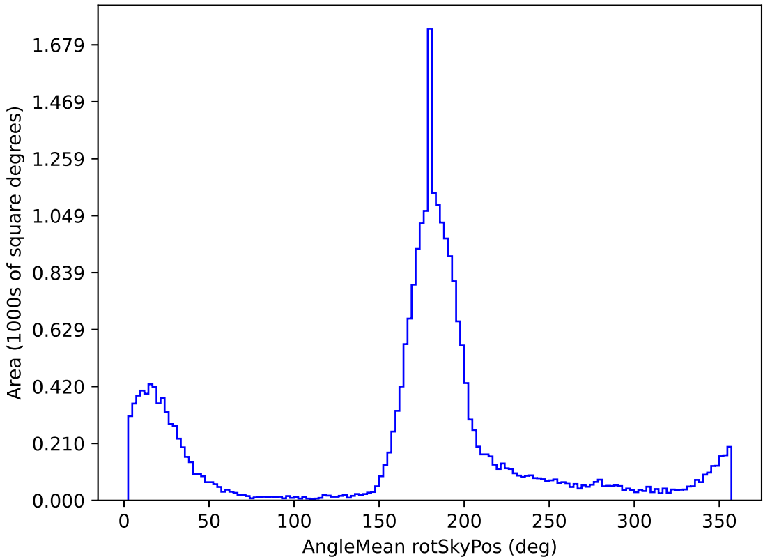
scp_reweight_v3.3_10yrs All sky g band: AngleMean rotSkyPos
