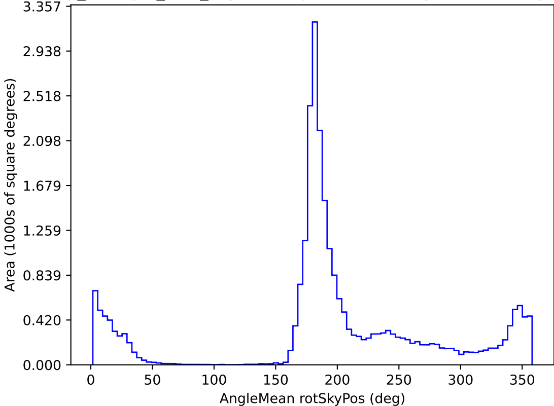
scp_reweight_v3.3_10yrs All sky all bands: AngleMean rotSkyPos
