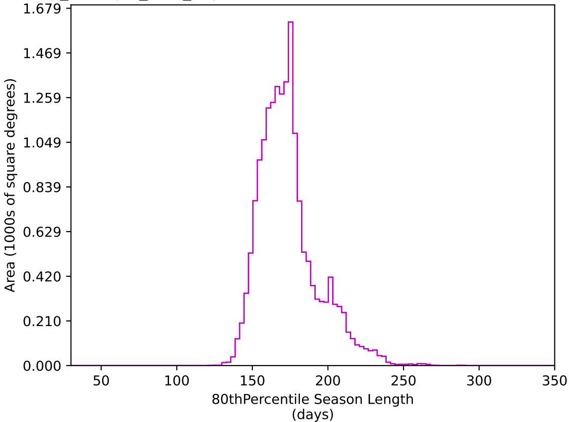
scp_reweight_v3.3_10yrs WFD z band: 80thPercentile Season Length
