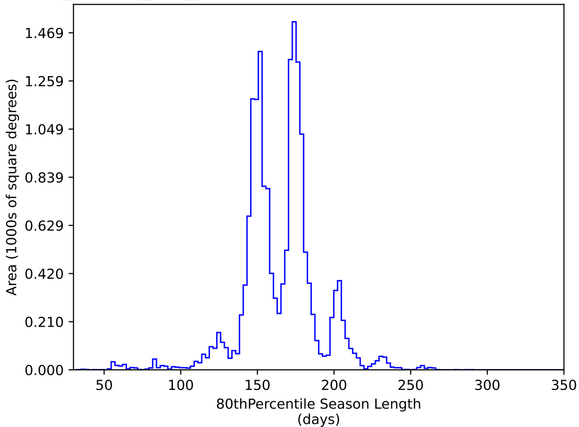
scp_reweight_v3.3_10yrs WFD y band: 80thPercentile Season Length
