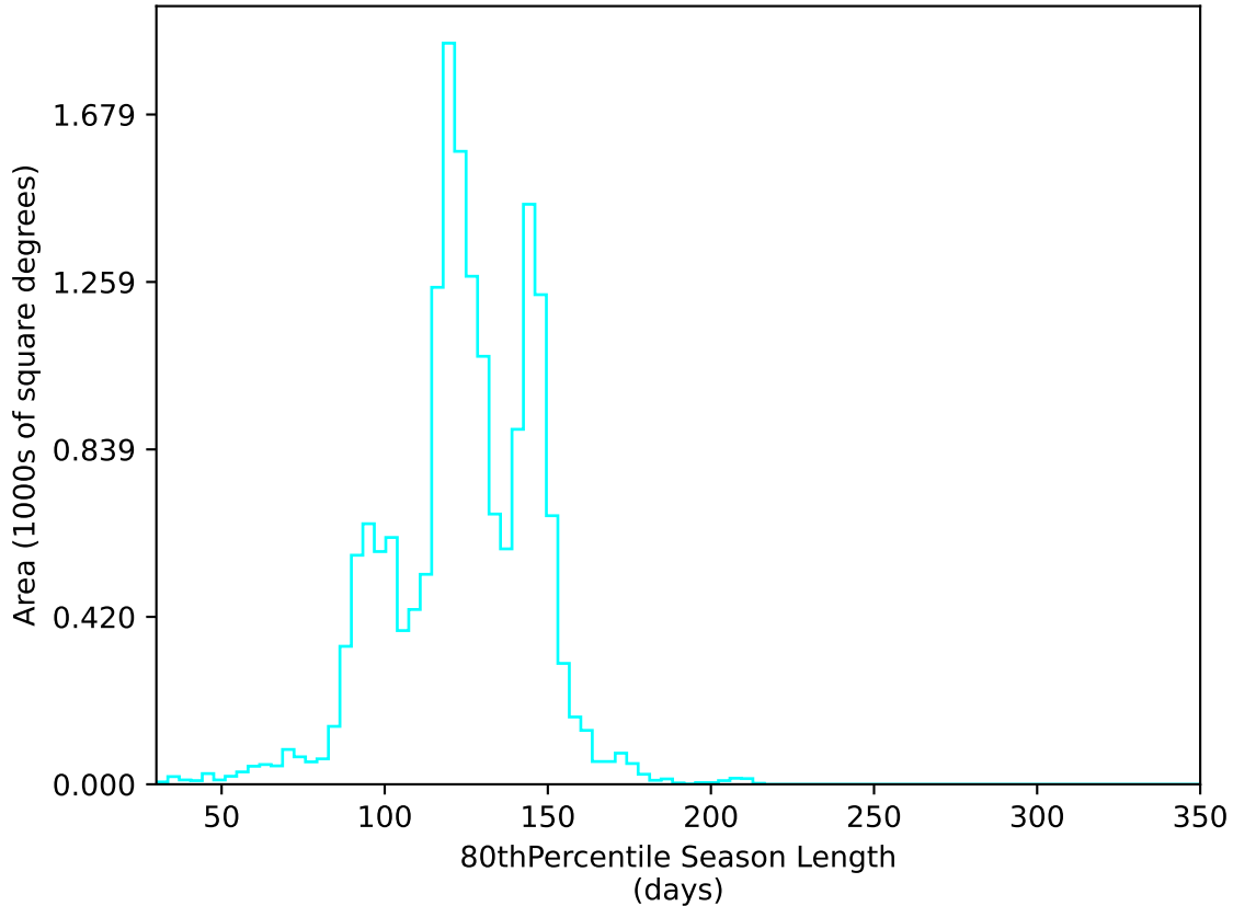
scp_reweight_v3.3_10yrs WFD u band: 80thPercentile Season Length
