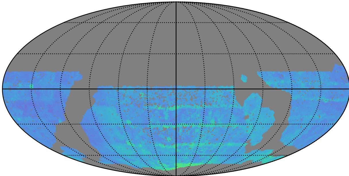
scp_reweight_v3.3_10yrs WFD r band: 80thPercentile Season Length
