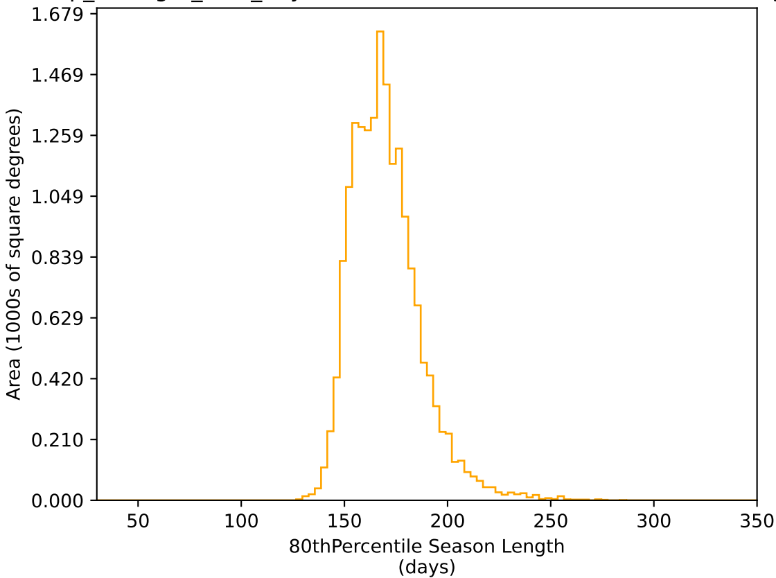
scp_reweight_v3.3_10yrs WFD r band: 80thPercentile Season Length
