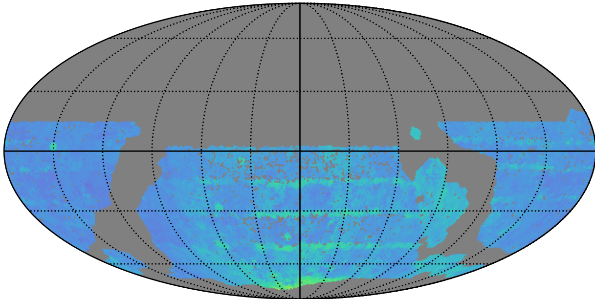
scp_reweight_v3.3_10yrs WFD i band: 80thPercentile Season Length
