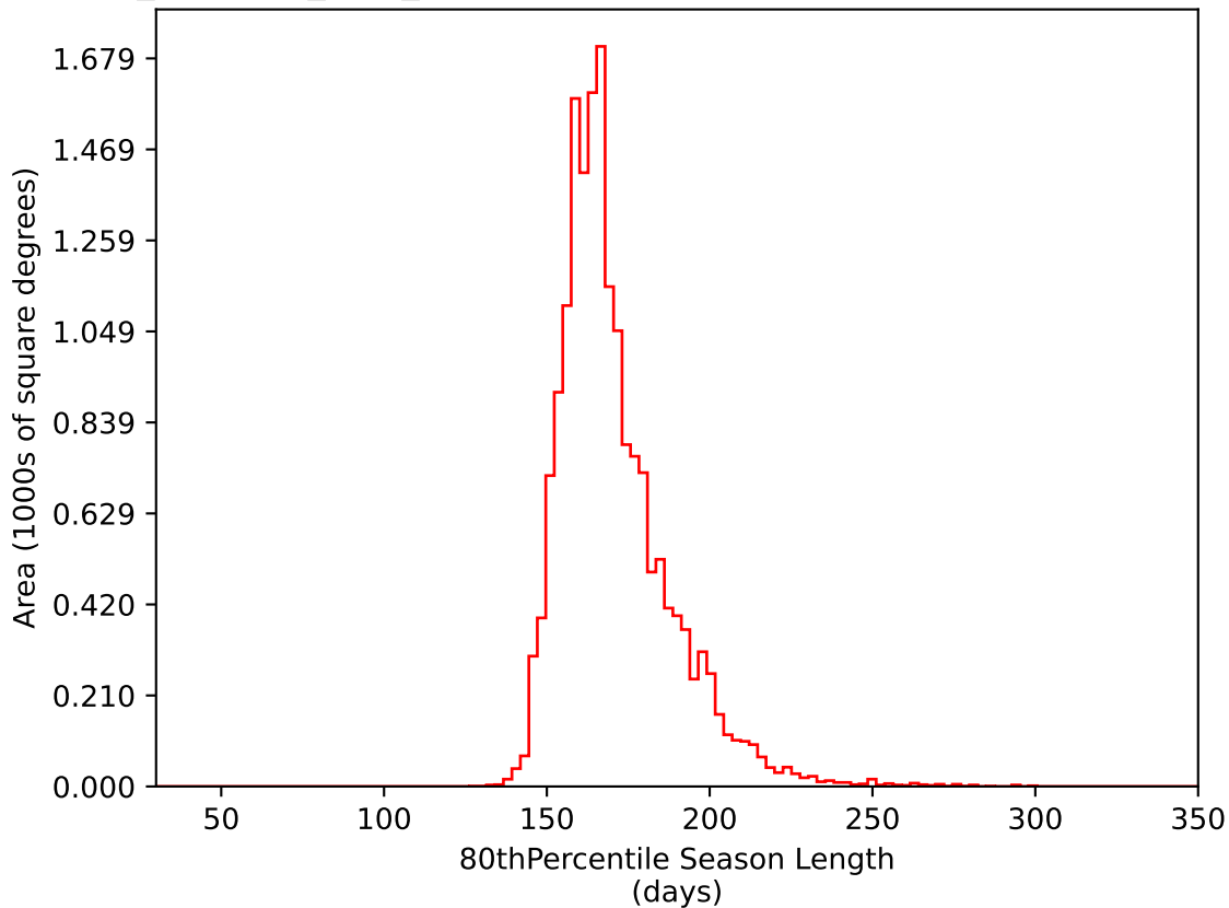
scp_reweight_v3.3_10yrs WFD i band: 80thPercentile Season Length
