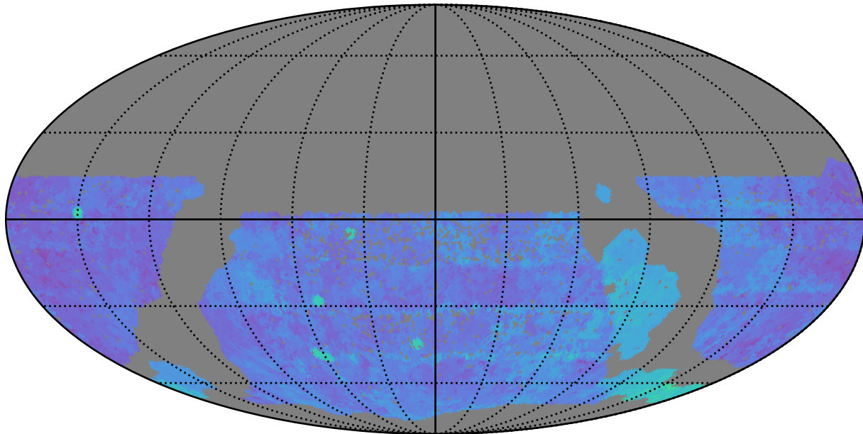
scp_reweight_v3.3_10yrs WFD g band: 80thPercentile Season Length
