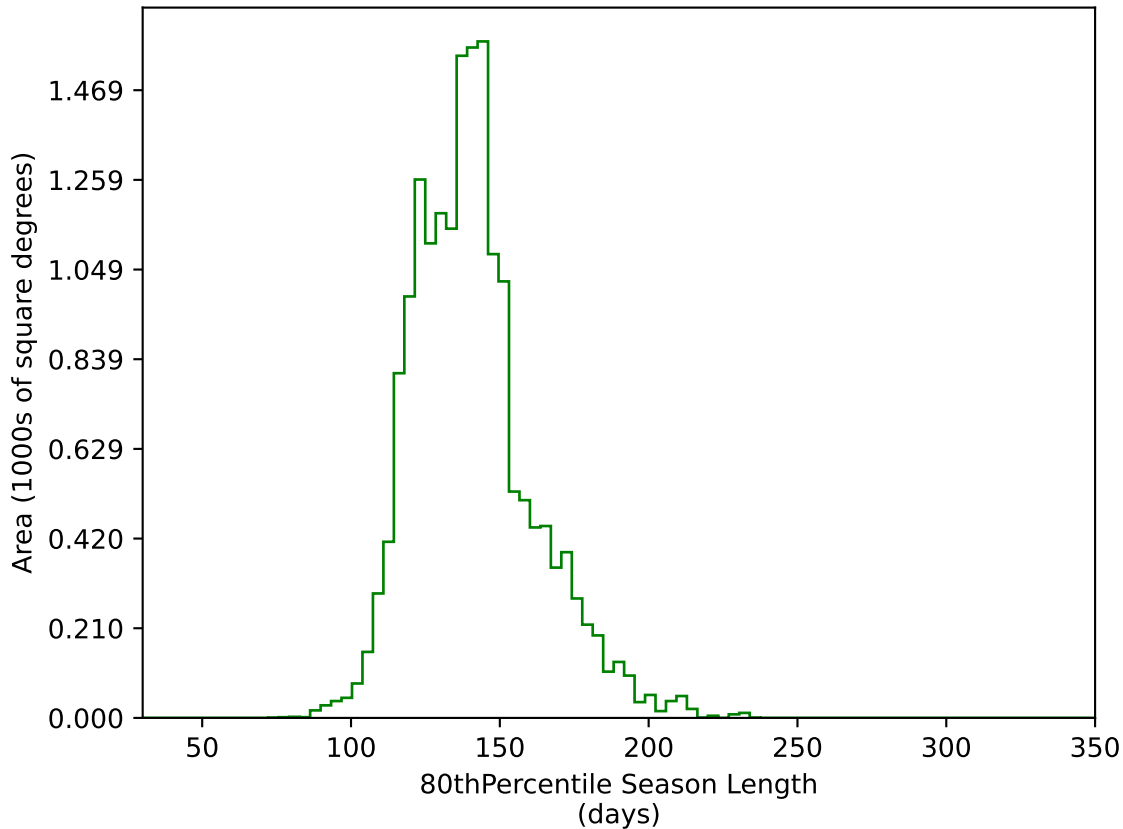
scp_reweight_v3.3_10yrs WFD g band: 80thPercentile Season Length
