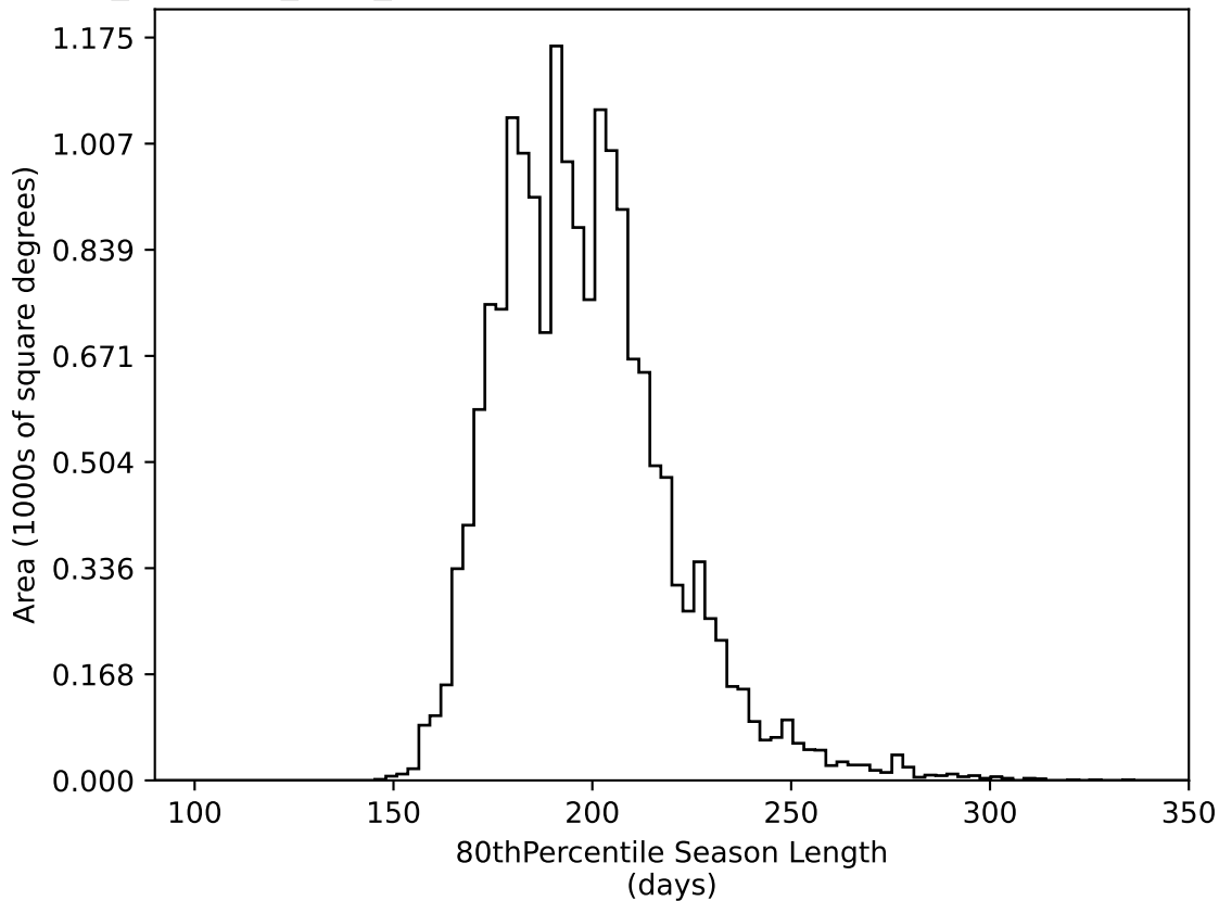
scp_reweight_v3.3_10yrs WFD all bands: 80thPercentile Season Length
