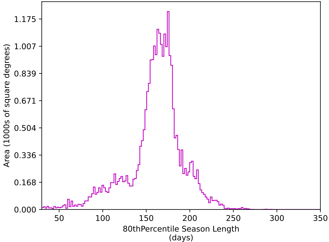
scp_reweight_v3.3_10yrs All sky z band: 80thPercentile Season Length
