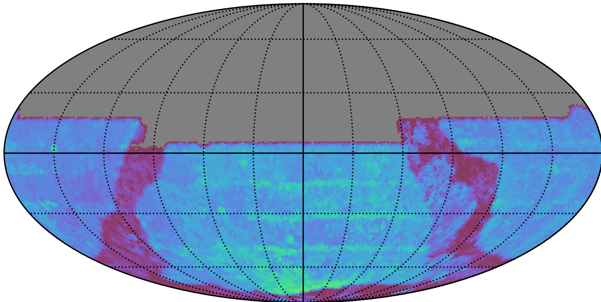
scp_reweight_v3.3_10yrs All sky y band: 80thPercentile Season Length
