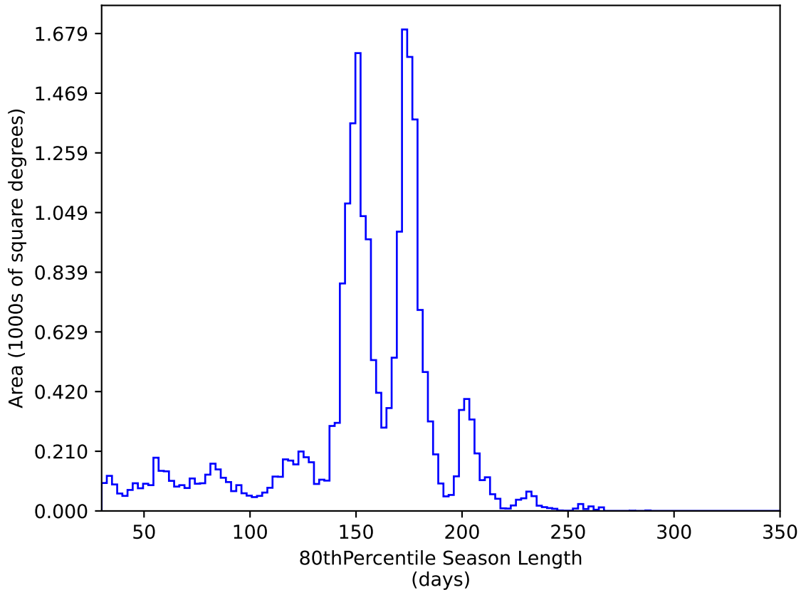
scp_reweight_v3.3_10yrs All sky y band: 80thPercentile Season Length
