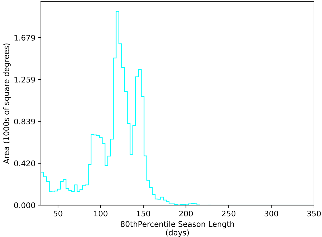
scp_reweight_v3.3_10yrs All sky u band: 80thPercentile Season Length
