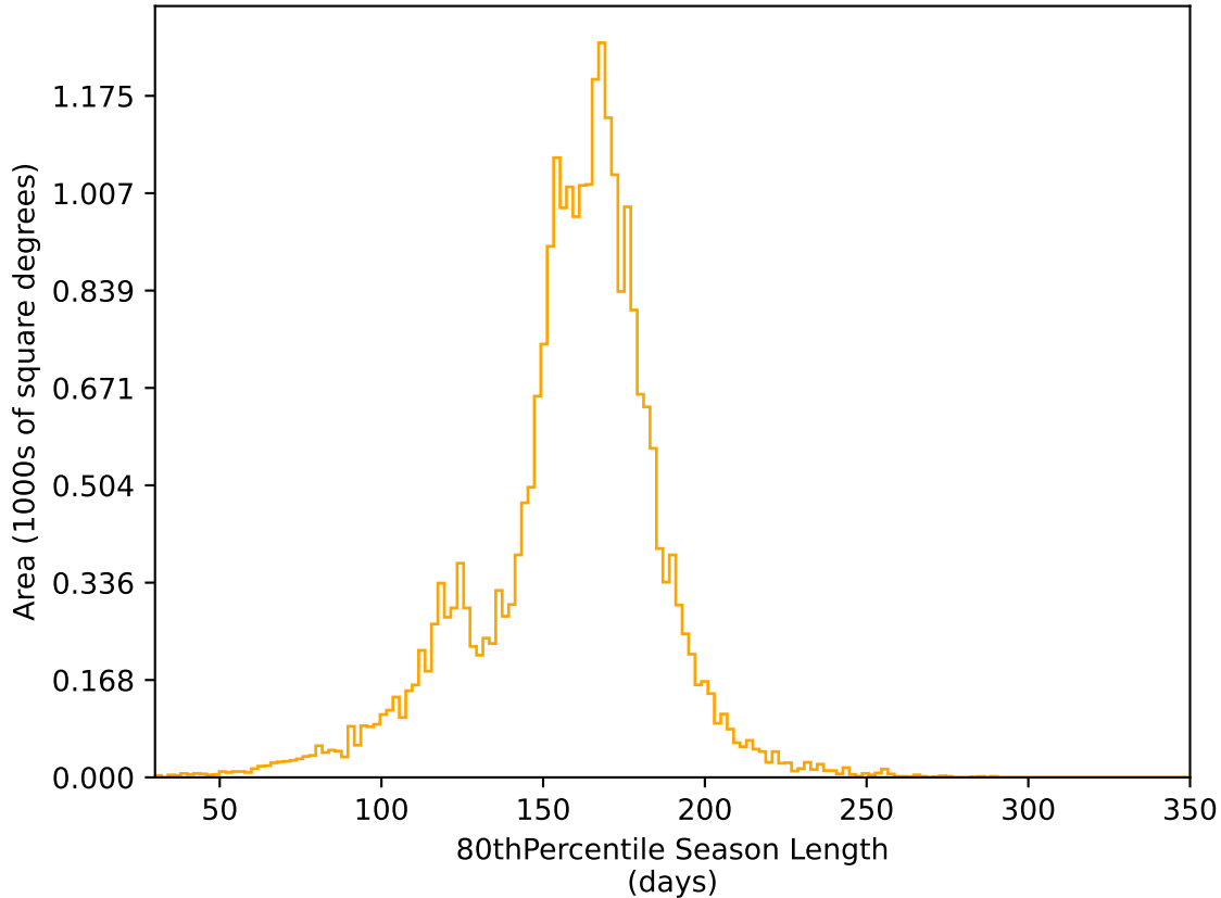
scp_reweight_v3.3_10yrs All sky r band: 80thPercentile Season Length
