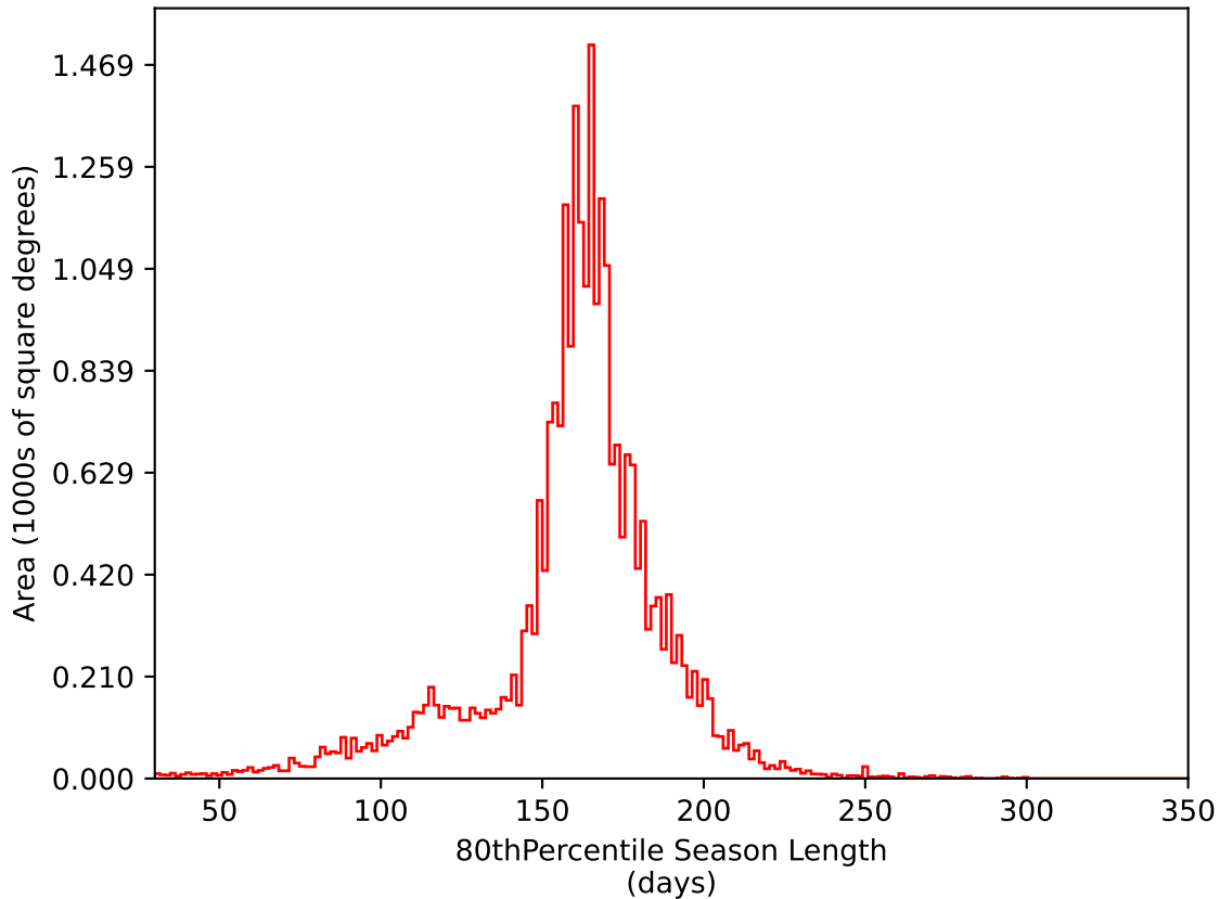
scp_reweight_v3.3_10yrs All sky i band: 80thPercentile Season Length
