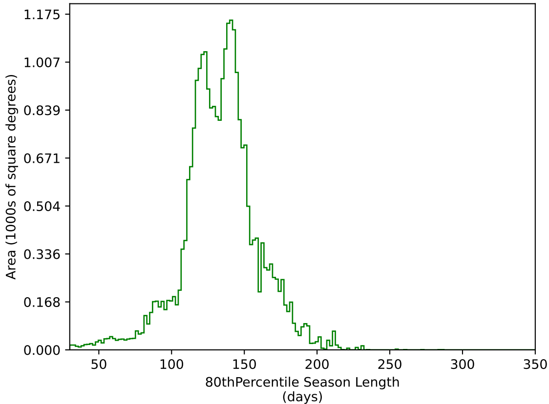
scp_reweight_v3.3_10yrs All sky g band: 80thPercentile Season Length
