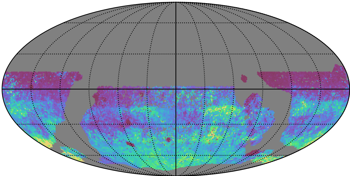
scp_reweight_v3.3_10yrs WFD zy bands: 75th Percentile Intranight Timespan
