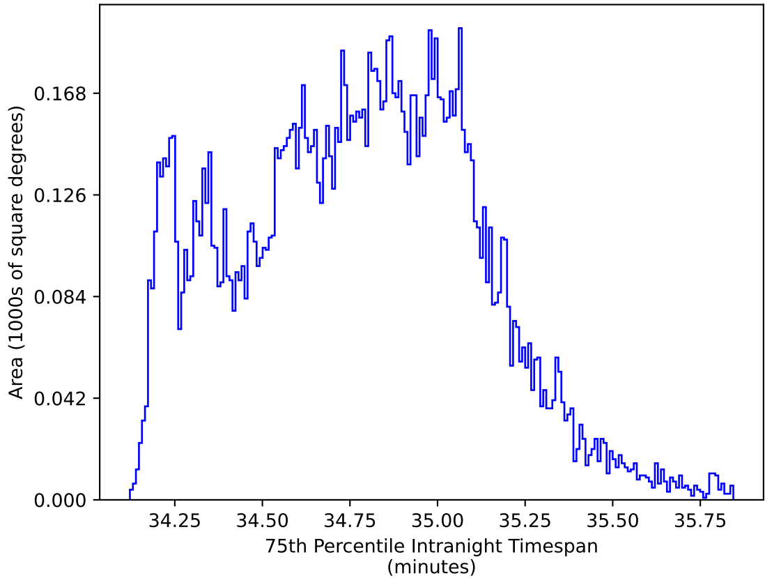
scp_reweight_v3.3_10yrs WFD zy bands: 75th Percentile Intranight Timespan
