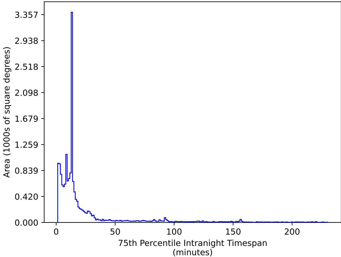
scp_reweight_v3.3_10yrs WFD z band: 75th Percentile Intranight Timespan
