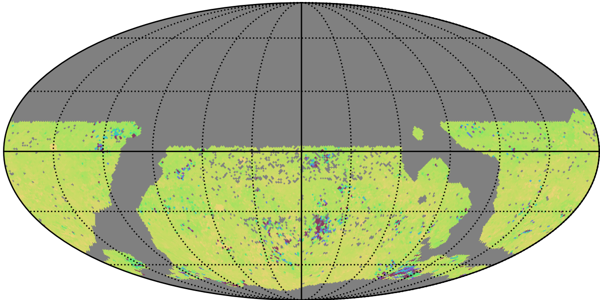
scp_reweight_v3.3_10yrs WFD ug bands: 75th Percentile Intranight Timespan
