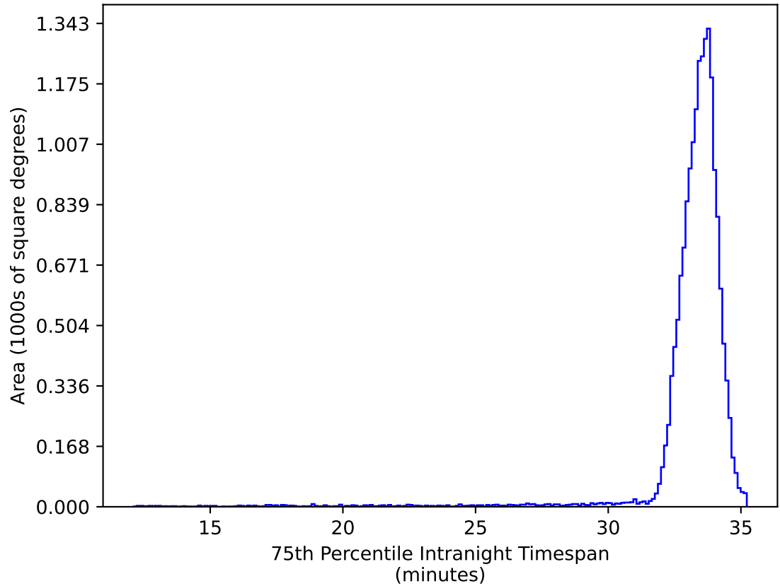
scp_reweight_v3.3_10yrs WFD ug bands: 75th Percentile Intranight Timespan
