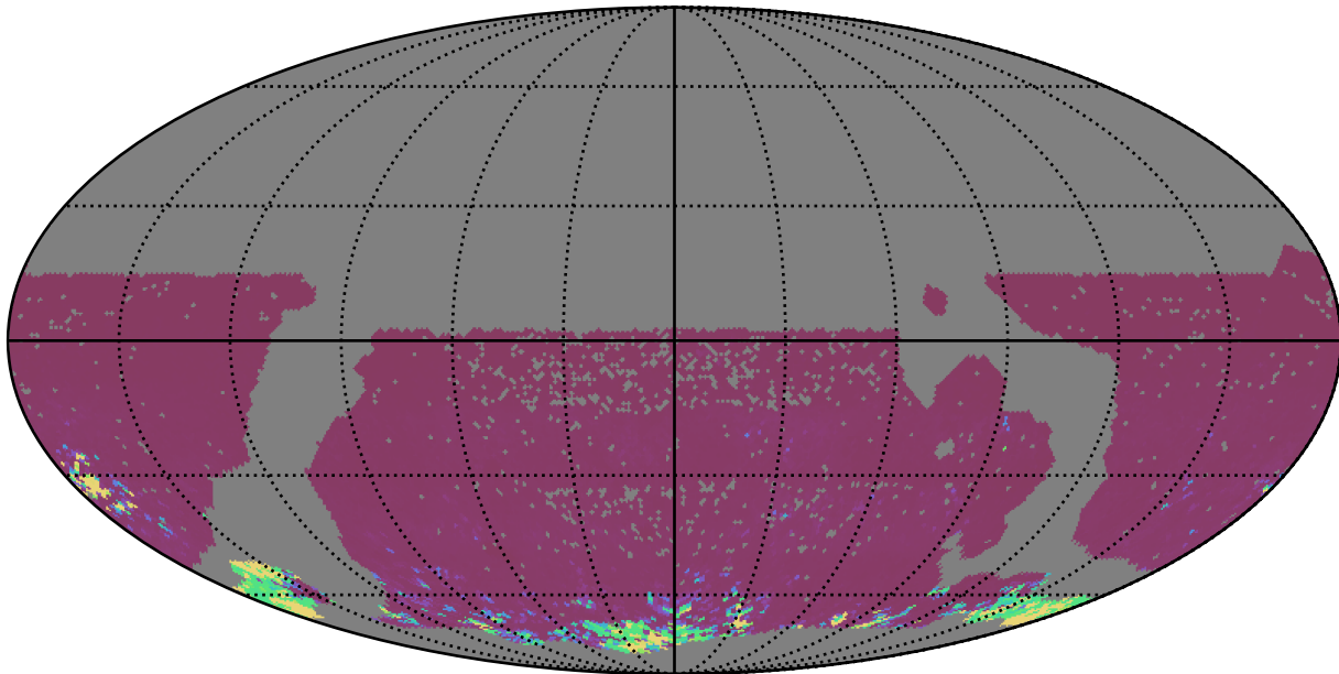
scp_reweight_v3.3_10yrs WFD ri bands: 75th Percentile Intranight Timespan
