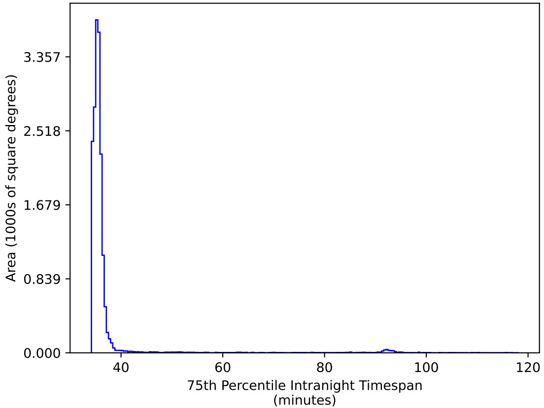
scp_reweight_v3.3_10yrs WFD ri bands: 75th Percentile Intranight Timespan
