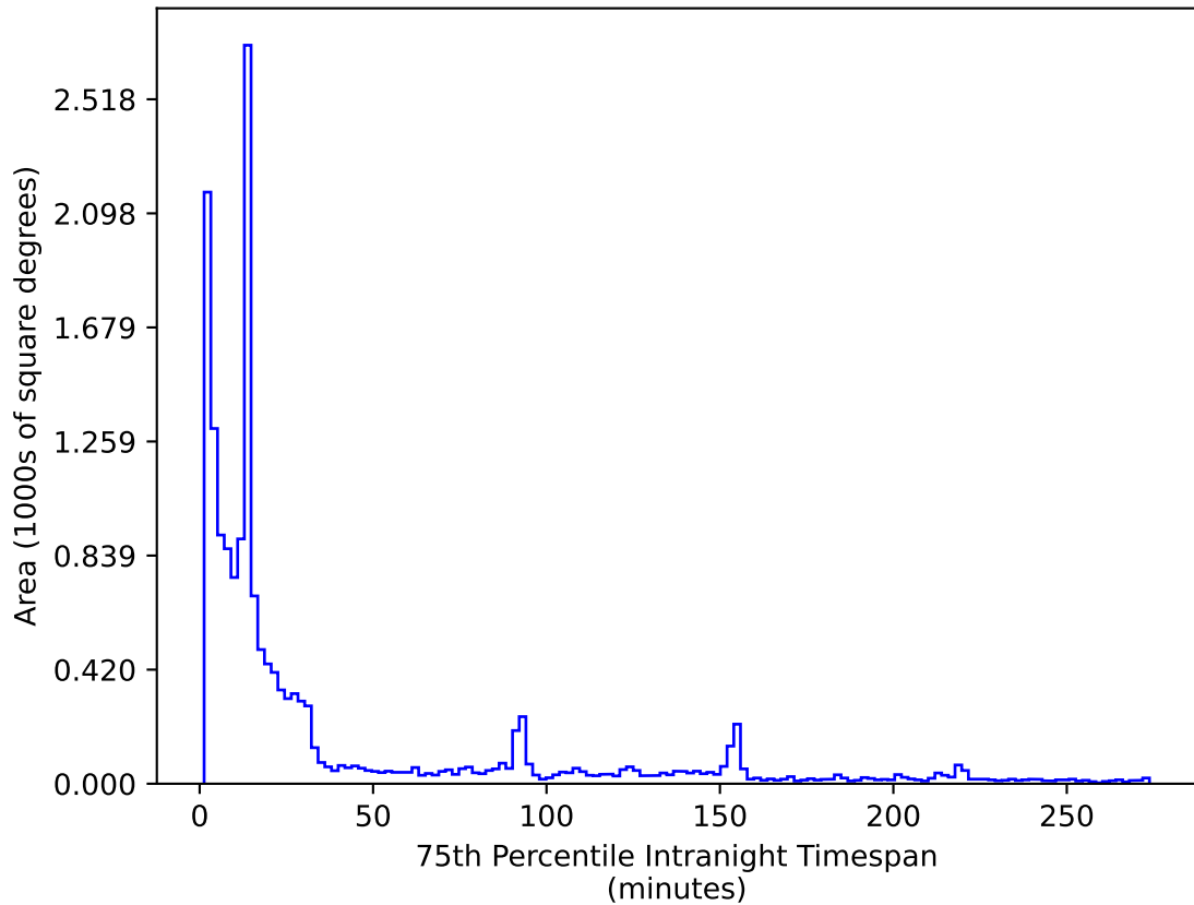
scp_reweight_v3.3_10yrs WFD r band: 75th Percentile Intranight Timespan
