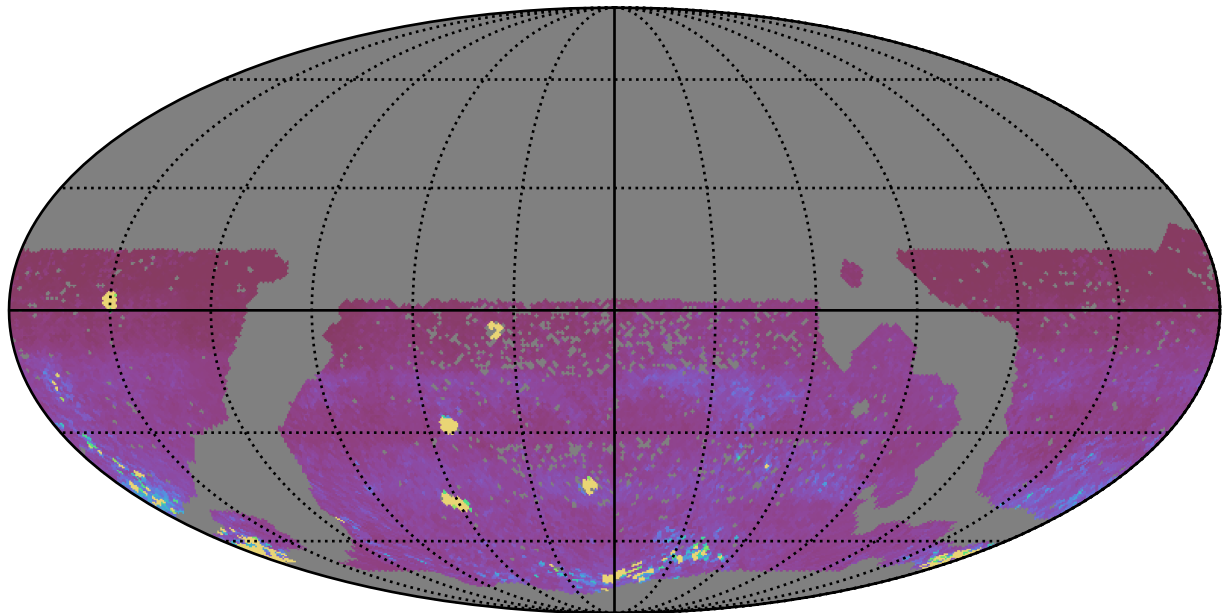
scp_reweight_v3.3_10yrs WFD iz bands: 75th Percentile Intranight Timespan
