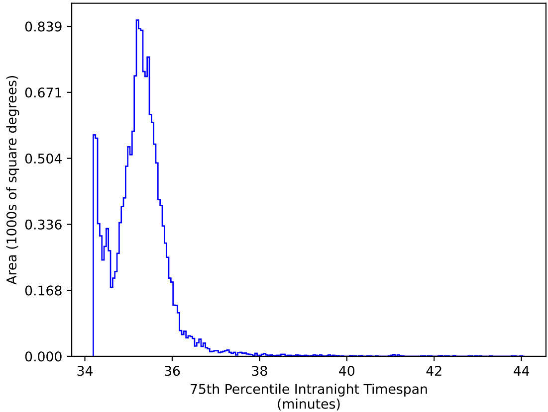
scp_reweight_v3.3_10yrs WFD iz bands: 75th Percentile Intranight Timespan
