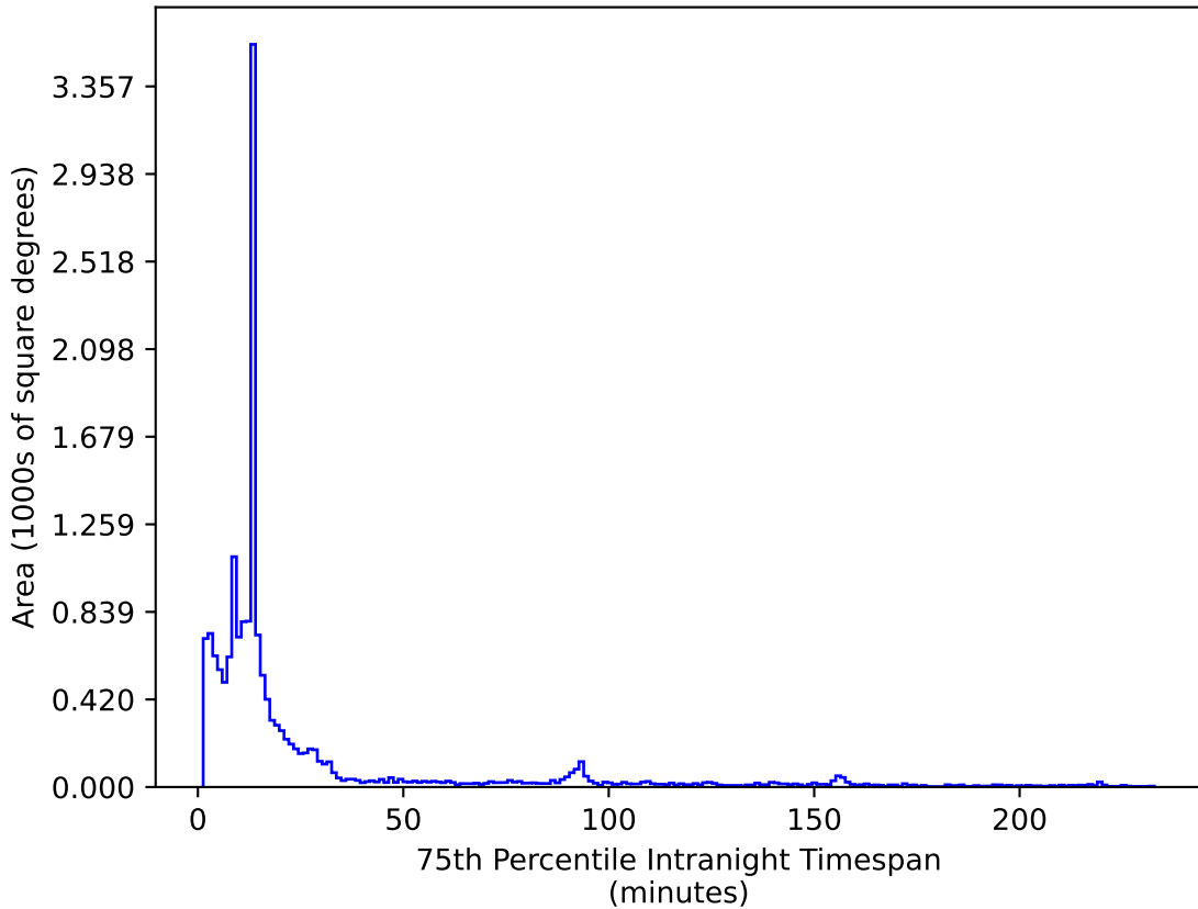
scp_reweight_v3.3_10yrs WFD i band: 75th Percentile Intranight Timespan
