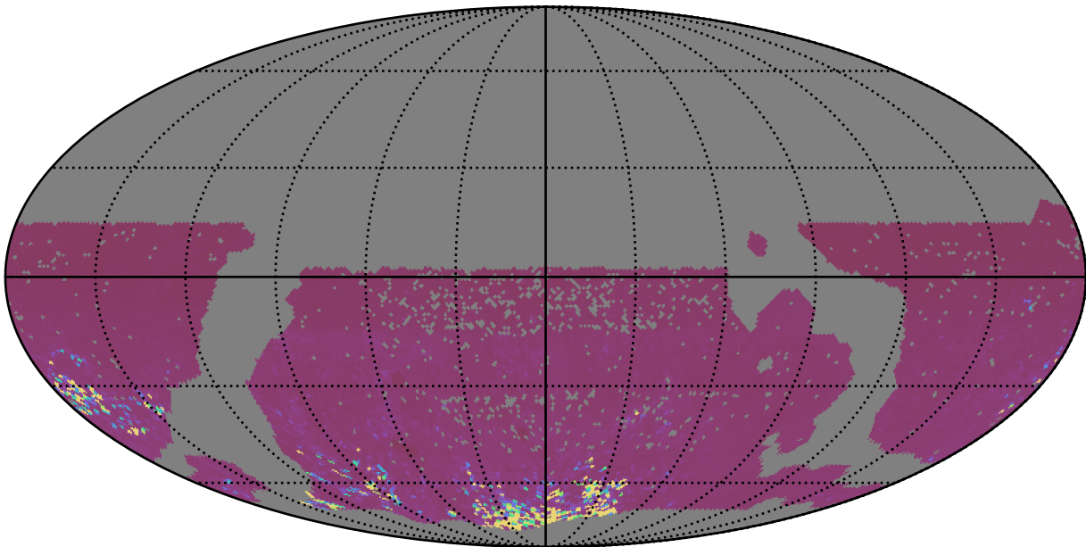
scp_reweight_v3.3_10yrs WFD gr bands: 75th Percentile Intranight Timespan
