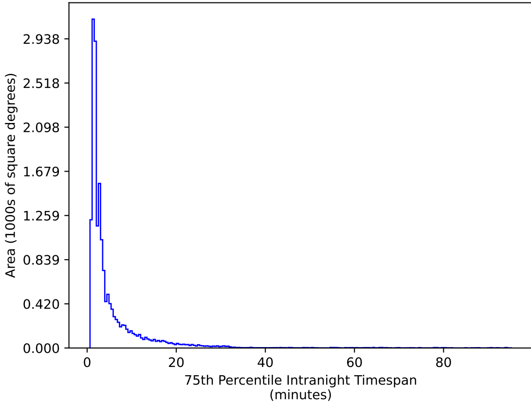
scp_reweight_v3.3_10yrs WFD g band: 75th Percentile Intranight Timespan
