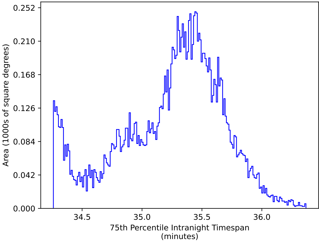
scp_reweight_v3.3_10yrs WFD: 75th Percentile Intranight Timespan
