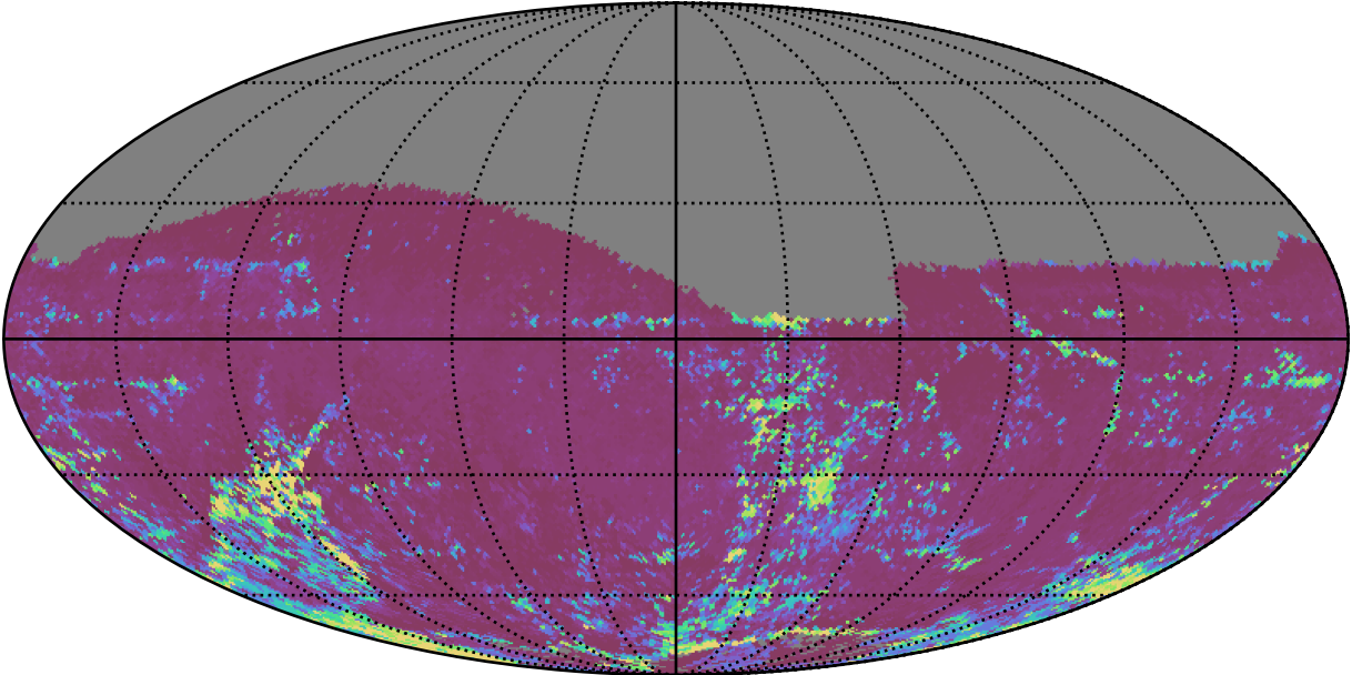
scp_reweight_v3.3_10yrs All sky z band: 75th Percentile Intranight Timespan
