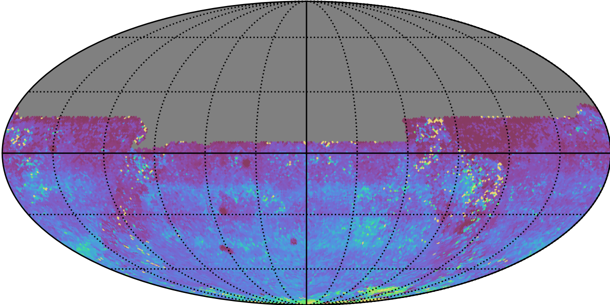
scp_reweight_v3.3_10yrs All sky y band: 75th Percentile Intranight Timespan
