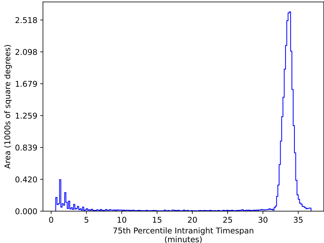
scp_reweight_v3.3_10yrs All sky ug bands: 75th Percentile Intranight Timespan
