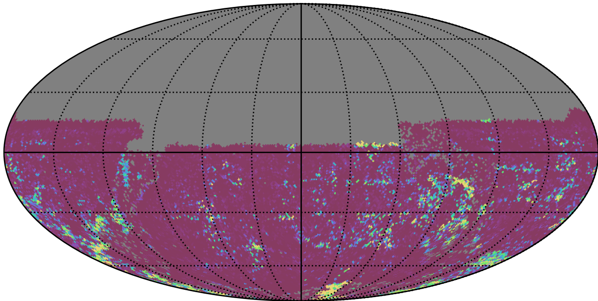
scp_reweight_v3.3_10yrs All sky u band: 75th Percentile Intranight Timespan
