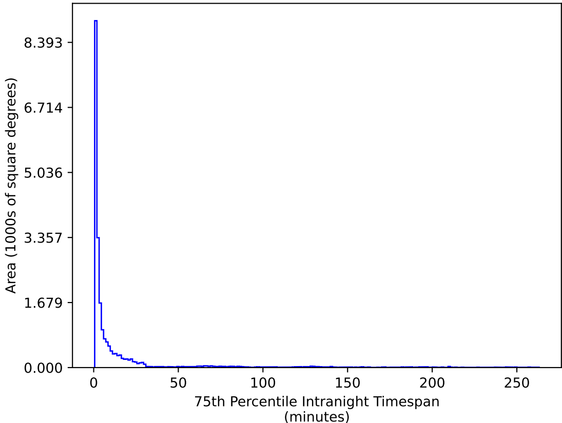
scp_reweight_v3.3_10yrs All sky u band: 75th Percentile Intranight Timespan
