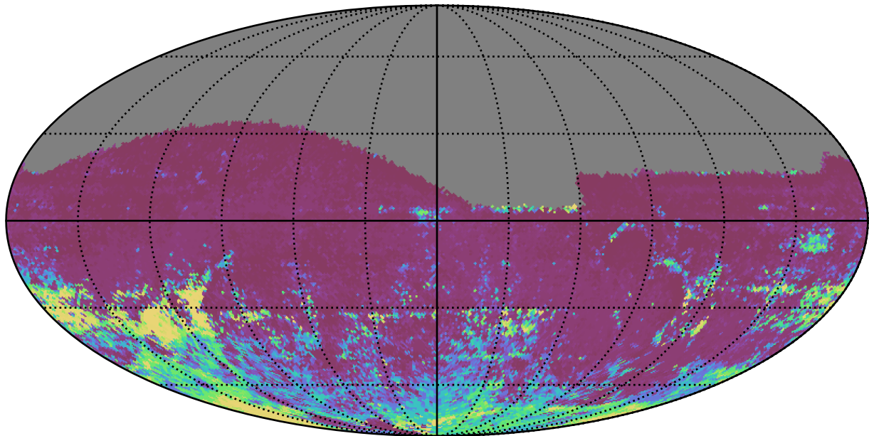
scp_reweight_v3.3_10yrs All sky r band: 75th Percentile Intranight Timespan
