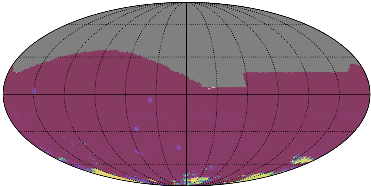
scp_reweight_v3.3_10yrs All sky iz bands: 75th Percentile Intranight Timespan
