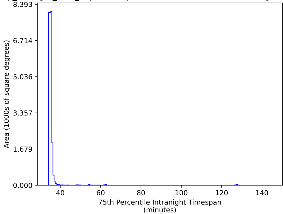
scp_reweight_v3.3_10yrs All sky iz bands: 75th Percentile Intranight Timespan
