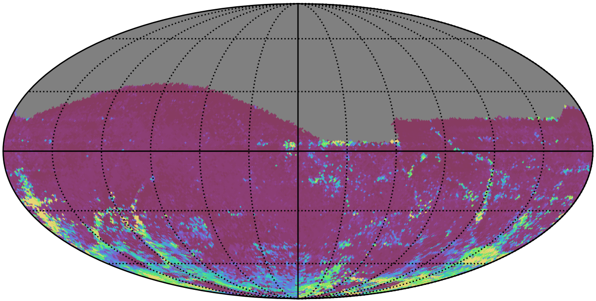
scp_reweight_v3.3_10yrs All sky i band: 75th Percentile Intranight Timespan
