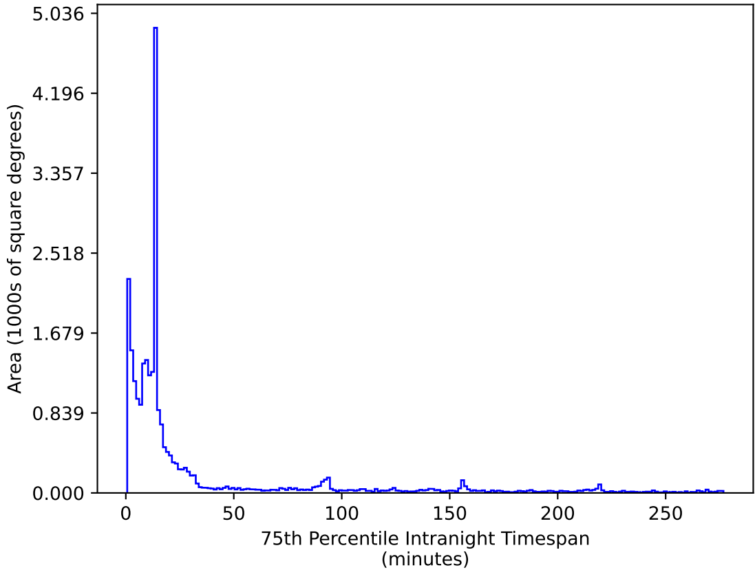
scp_reweight_v3.3_10yrs All sky i band: 75th Percentile Intranight Timespan
