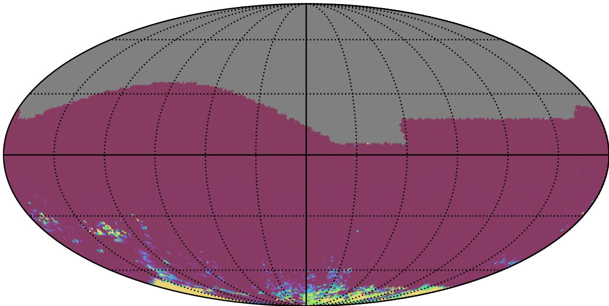
scp_reweight_v3.3_10yrs All sky gr bands: 75th Percentile Intranight Timespan
