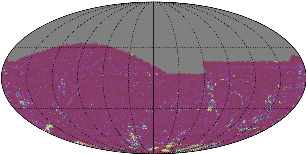
scp_reweight_v3.3_10yrs All sky g band: 75th Percentile Intranight Timespan
