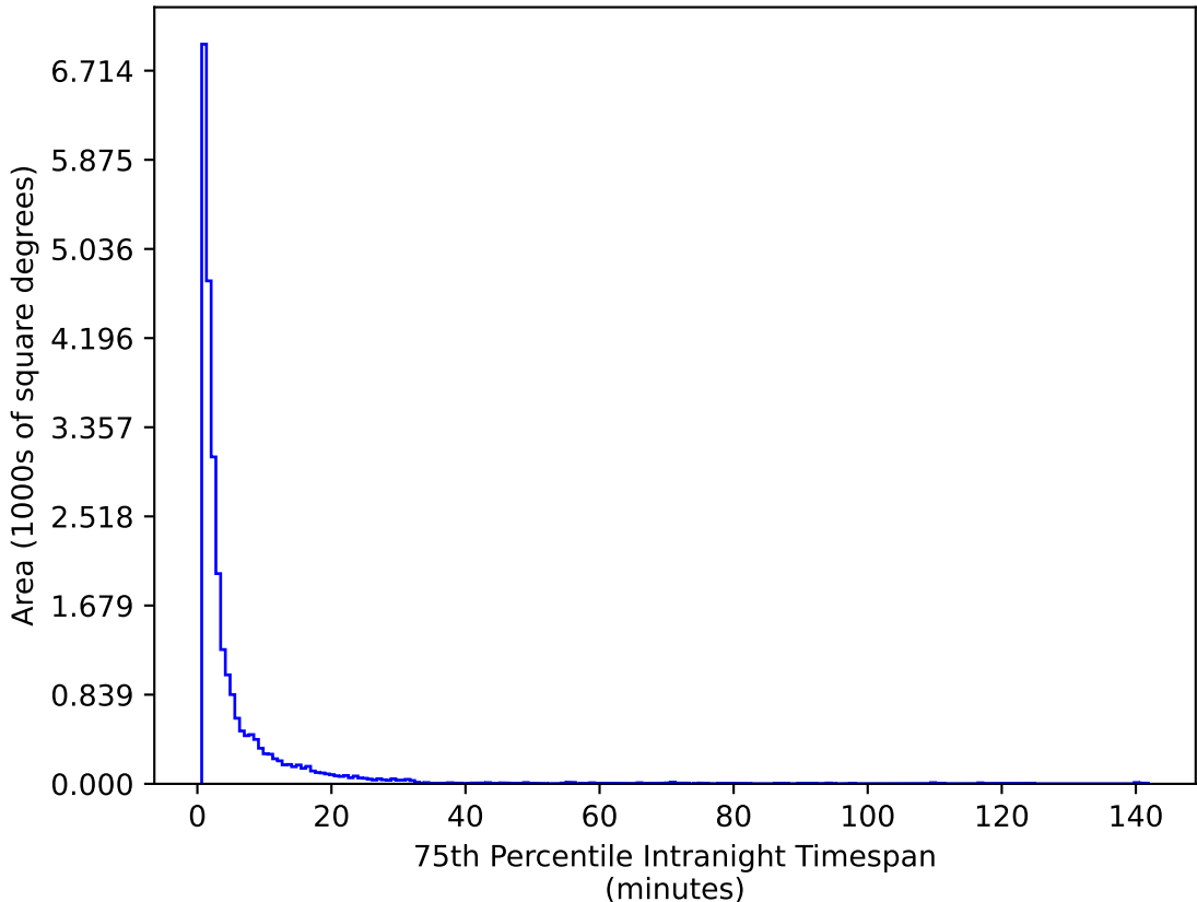
scp_reweight_v3.3_10yrs All sky g band: 75th Percentile Intranight Timespan
