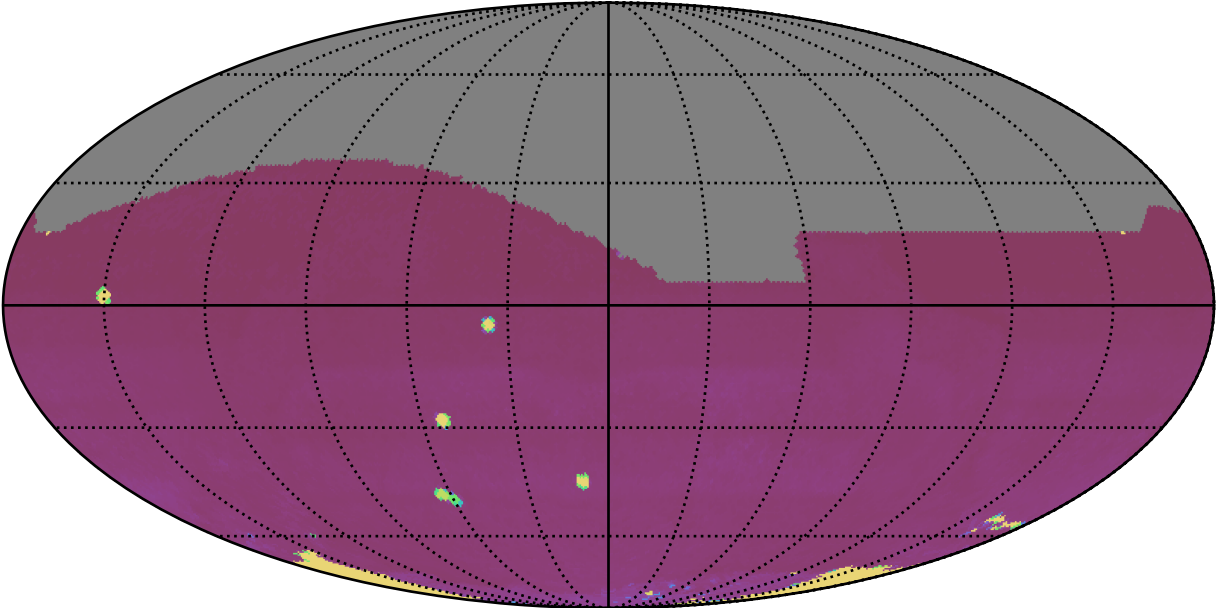
scp_reweight_v3.3_10yrs All sky all bands: 75th Percentile Intranight Timespan
