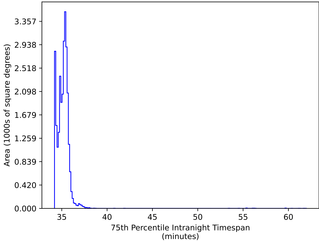
scp_reweight_v3.3_10yrs All sky all bands: 75th Percentile Intranight Timespan
