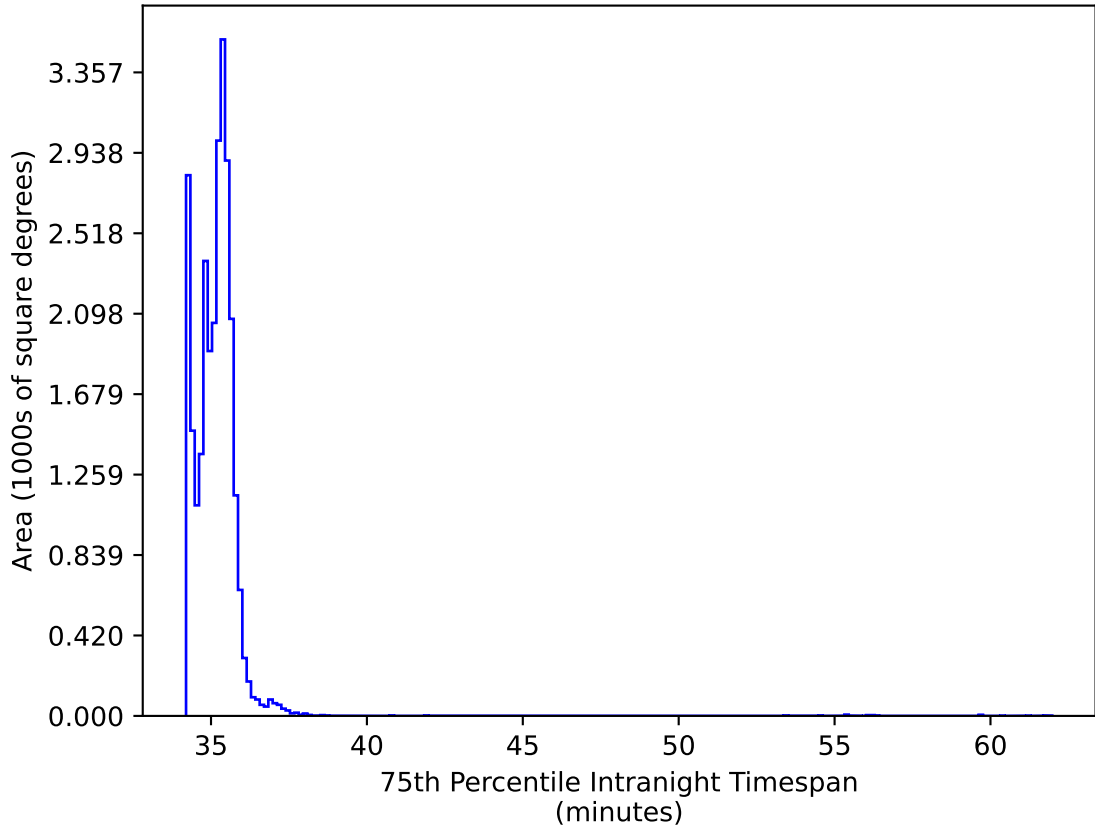
scp_reweight_v3.3_10yrs All sky: 75th Percentile Intranight Timespan
